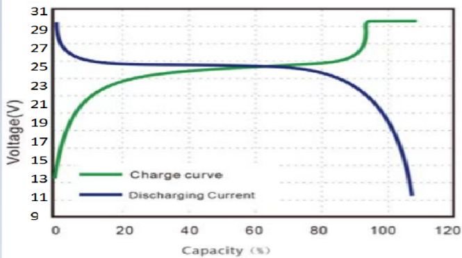
● Charge and discharge curve@0.5C 25°C
